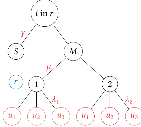
Figure 6. The nested logit structure.
